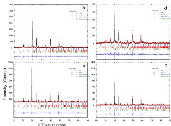
Figure 25. \text{Yb}_2\text{V}_2\text{O}_7 PXRD Patterns and the Rietveld Analyses of (a) S1, (b) S2, (c) S3, and (d) S4.
