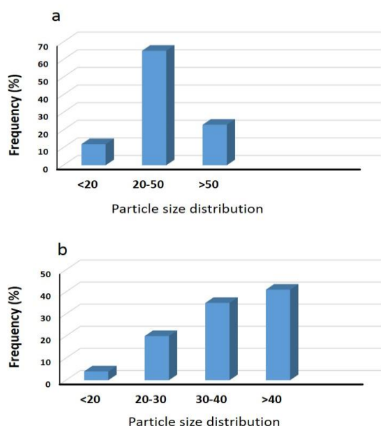
Figure 4. Particle size distribution of pure \text{Mn}_3\text{O}_4 (a) and 8% Gd-doped \text{Mn}_3\text{O}_4 (b)
