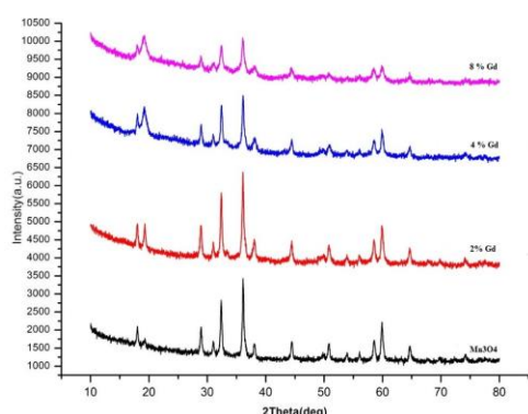
Figure 1. P-XRD pattern of manganese oxide doped with gadolinium cation \text{Mn}_{3-x}\text{Gd}_x\text{O}_4 ( x=0 to x=0.08 )
