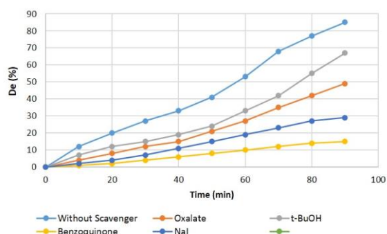
Figure 7. The effects of different inhibitors on the color removal efficiency under the following conditions: [dye] = 20 mg/L, [Catalyst] = 1 g/L, [Scavenger] = 5 mM
