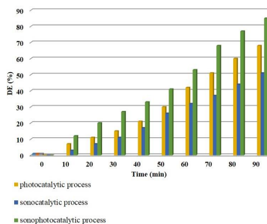
Figure 5. Comparison of different processes in the removal of methylene blue dye considering the following conditions: [Dye] = 20 mg/L, [Catalyst] = 1 g/L.
