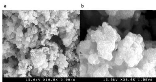
Figure 3. SEM image of nanoparticles synthesized with the chemical formula \text{Mn}_{3-x}\text{Gd}_x\text{O}_4 ( x=0 (a), x=0.08 (b))
