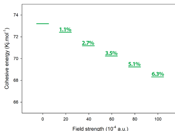
Figure 3. Cohesive energy values at different electric field intensities.
