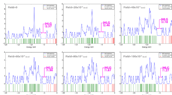
Figure 4. DOS plot of the studied structure in the intensity of different field effect.
