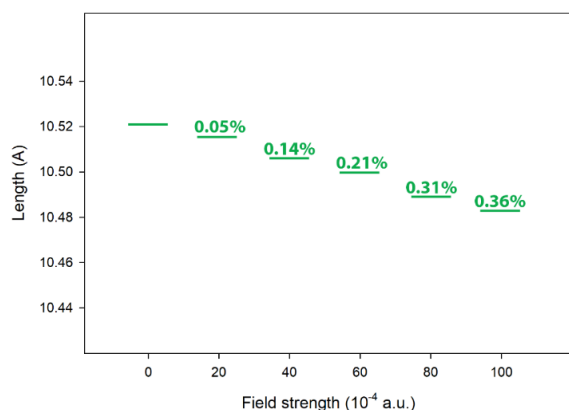
Figure 2. Changes in the length of the molecule in the intensity of different electric fields (zero electric field was used as a reference).
