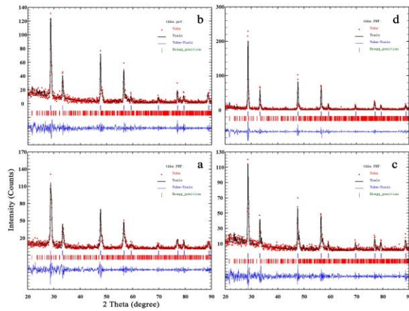
Figure 1. X-Ray diffraction patterns and the rietveld analyses of a) S_1 , b) S_2 , c) S_3 and d) S_4 .
