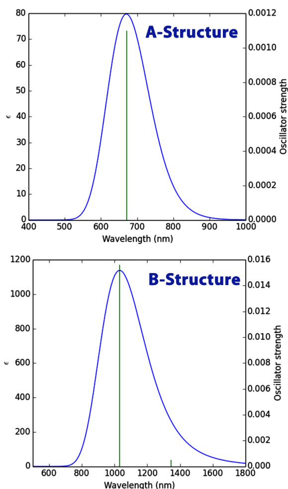
Figure 4. The UV spectrum of the designed structures using the method TD/DFT/CAM-B3LYP/6-311+G(d,p).
