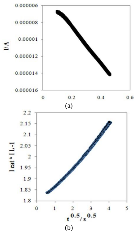
Figure 3. (a) Current dependence on t^{-1/2} . (b) Dependence of I_{\text{cat}}/I_L on t^{1/2} from the data of chronoamperograms related to the concentration of 0 mM and mM2 in figure (2-3).
