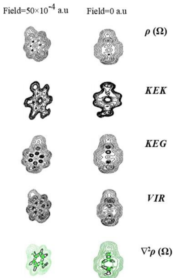
Figure 5. 1. The external EF (along the x-axis, all in a.u unit) effect on local/atomic electronic contour maps of local electron density, \rho ( \Omega ), local electronic kinetic energy, KEK , atomic lagrangian kinetic energy, KEG local potential/virial energy/force, VIR ( \Omega ), and local laplacian of electron density, \nabla^2 \rho ( \Omega ), of the paracetamol molecular system, Fig.4(a), are calculated using AIM theory.
