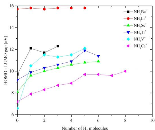
Fig. 7. (Color online) energy gap between highest occupied and lowest unoccupied molecular orbital for \text{NH}_2\text{M}^+(\text{nH}_2) , where M is Be, Li, Sc, Ti, V, and Ca (MP2/6-311++G(d, p) level).
