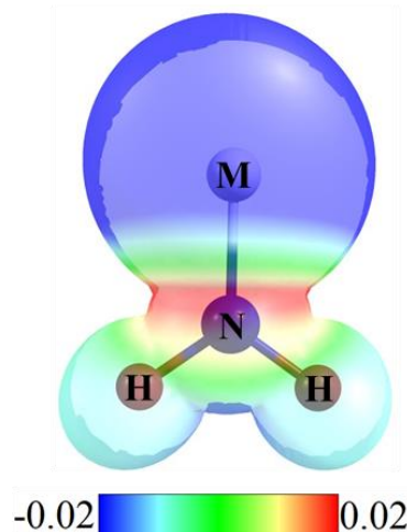
Fig. 3. The presentation MEP surface of the \text{NH}_2\text{M}^+ compound, the surfaces are specified by the 0.0004 electrons/b3 contour of an electronic density and color ranges in a.u.
