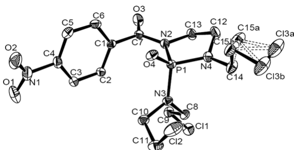
Fig. 1 Molecular structure of DIAZ compound, showing 50% probability displacement ellipsoids.
